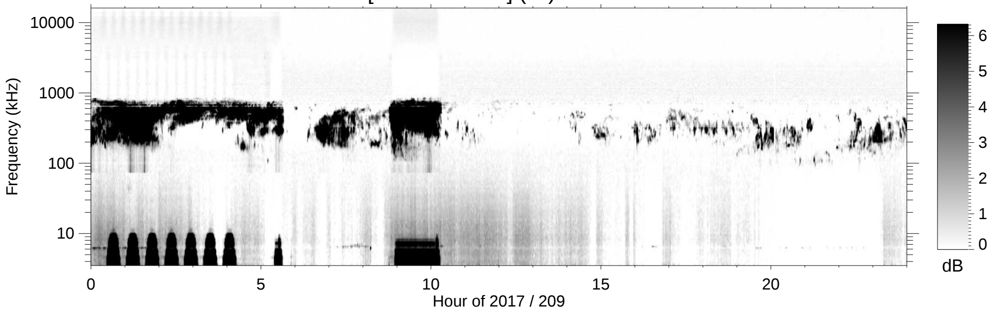
RPWS [ABCH1H2/Ex] (-B) 2017/07/28
