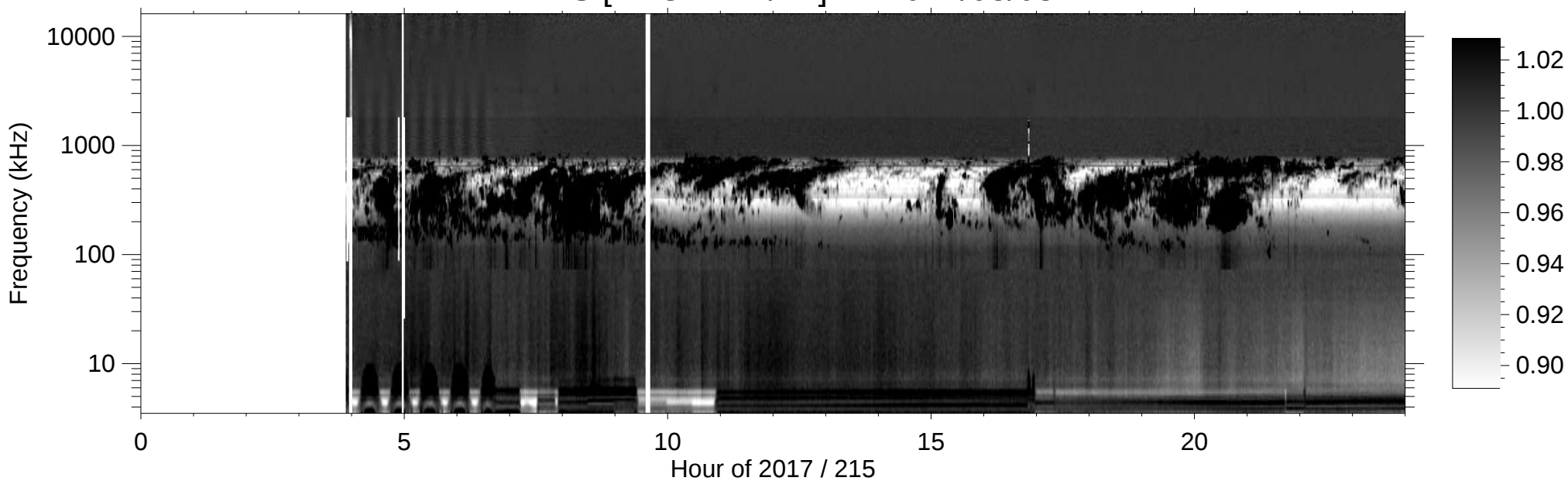
RPWS [ABCH1H2/Ex] (-B) 2017/08/03
