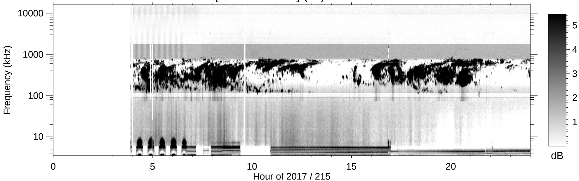
RPWS [ABCH1H2/Ex] (-B) 2017/08/03
