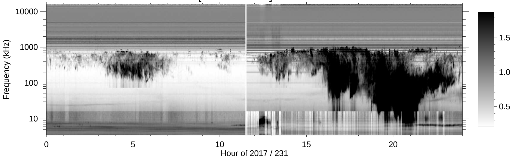
RPWS [ABCH1H2/Ex] (-B) 2017/08/19
