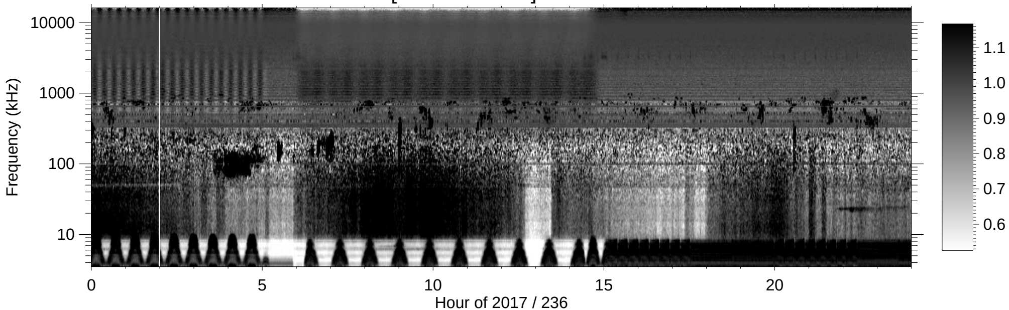
RPWS [ABCH1H2/Ex] (-B) 2017/08/24
