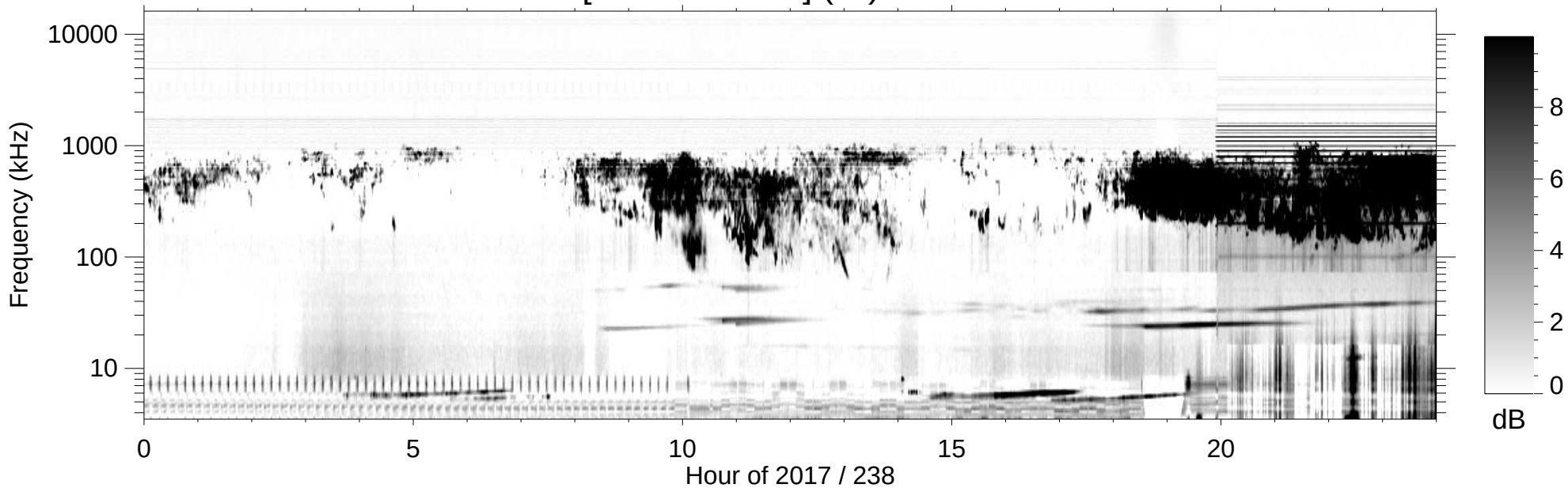
RPWS [ABCH1H2/Ex] (-B) 2017/08/26
