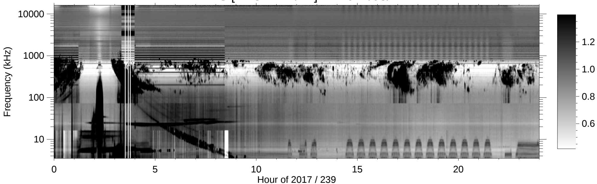
RPWS [ABCH1H2/Ex] (-B) 2017/08/27
