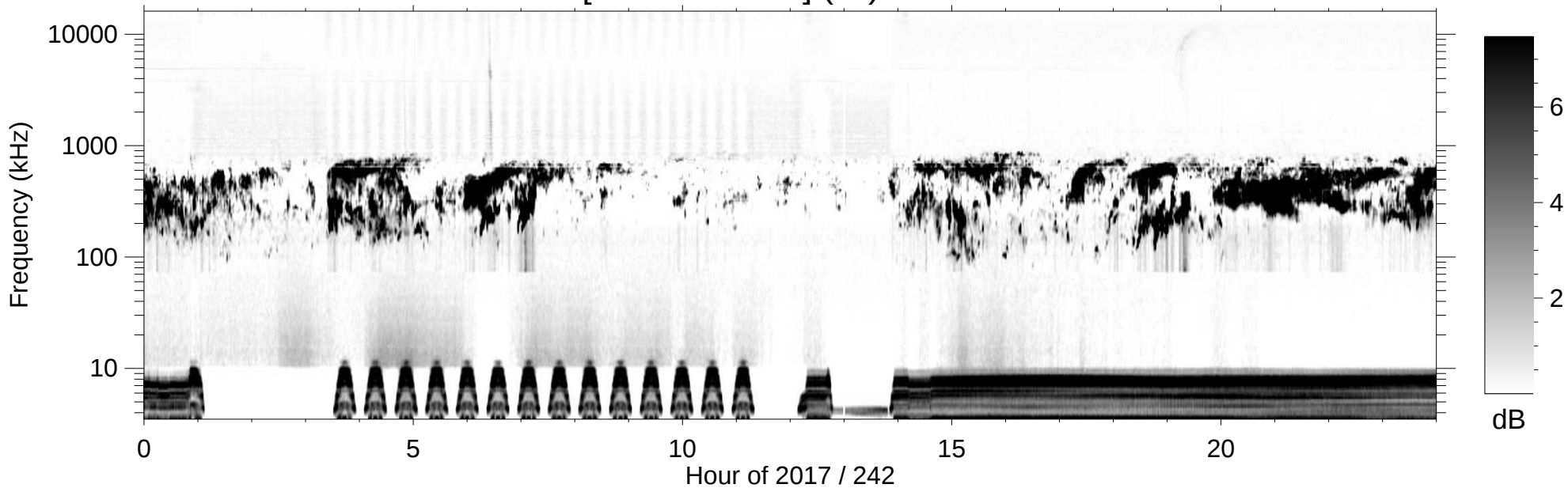
RPWS [ABCH1H2/Ex] (-B) 2017/08/30
