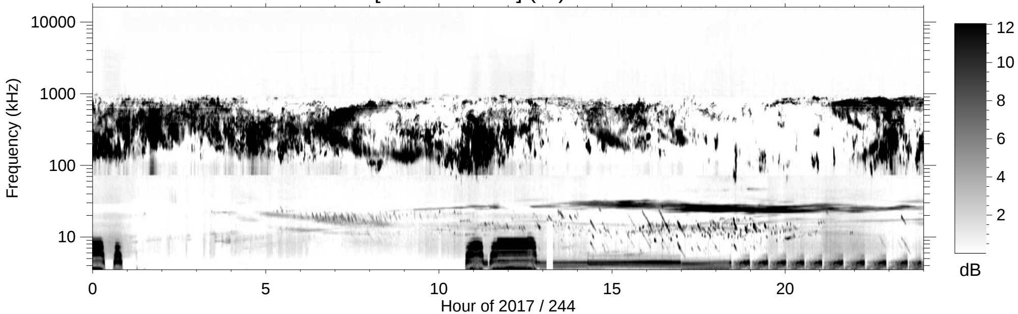
RPWS [ABCH1H2/Ex] (-B) 2017/09/01
