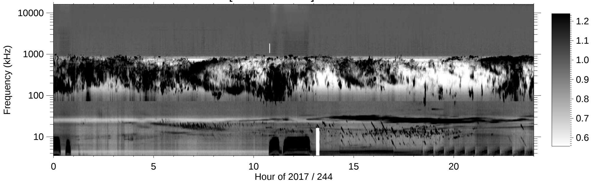
RPWS [ABCH1H2/Ex] (-B) 2017/09/01
