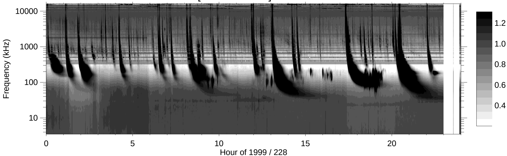
RPWS [ABCH1H2/Ex] (-B) 1999/08/16
