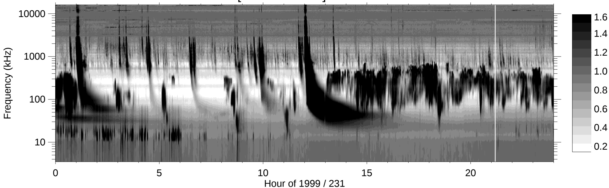
RPWS [ABCH1H2/Ex] (-B) 1999/08/19
