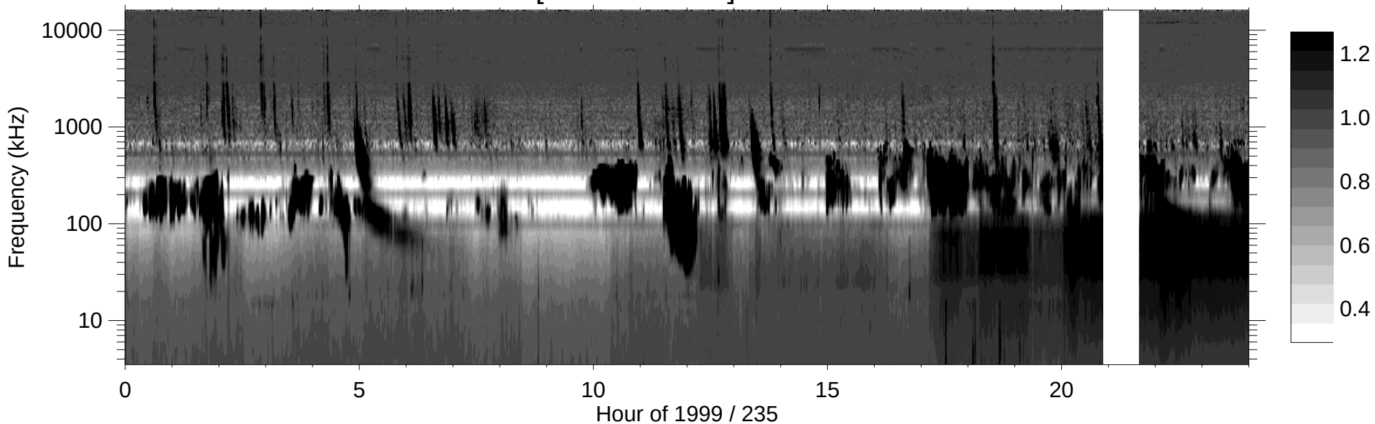
RPWS [ABCH1H2/Ex] (-B) 1999/08/23
