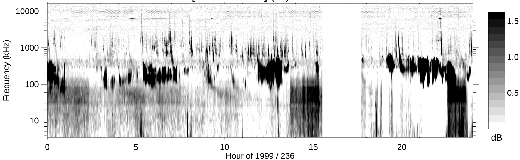
RPWS [ABCH1H2/Ex] (-B) 1999/08/24
