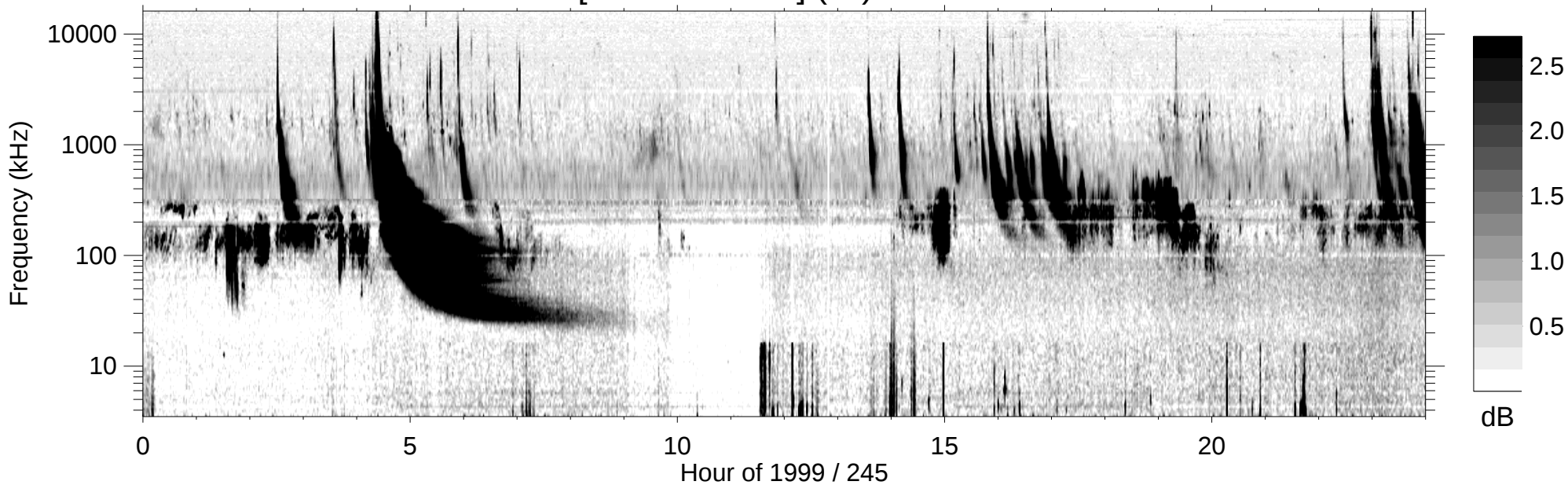
RPWS [ABCH1H2/Ex] (-B) 1999/09/02
