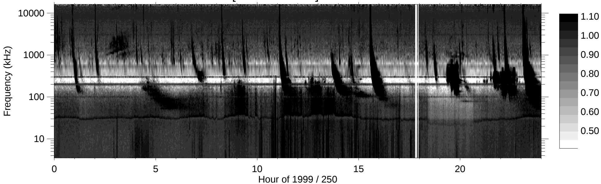
RPWS [ABCH1H2/Ex] (-B) 1999/09/07
