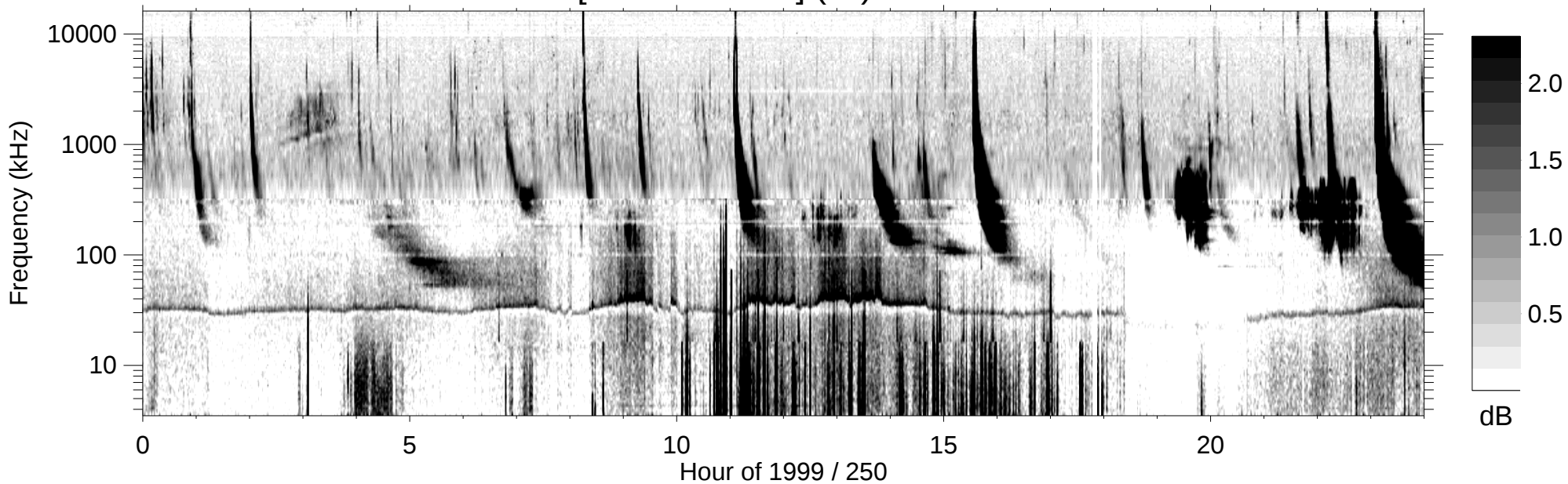
RPWS [ABCH1H2/Ex] (-B) 1999/09/07
