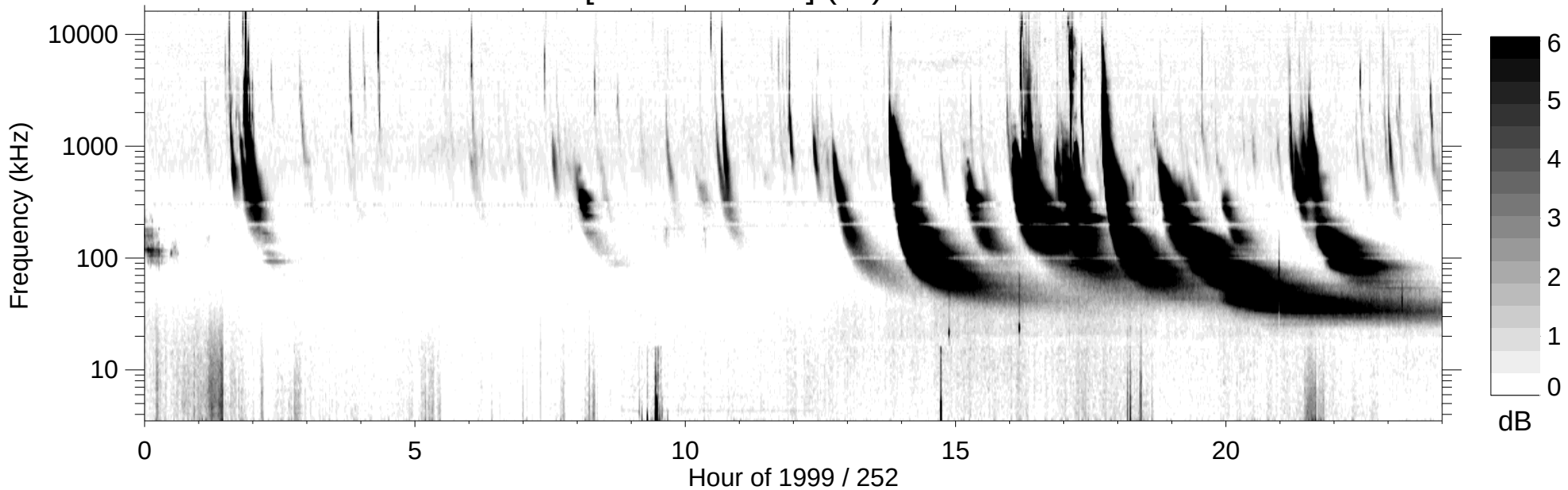
RPWS [ABCH1H2/Ex] (-B) 1999/09/09
