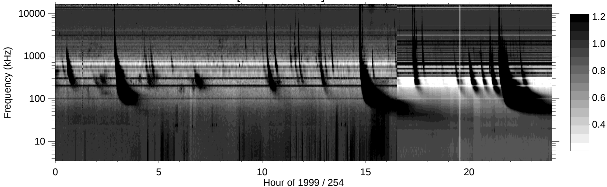
RPWS [ABCH1H2/Ex] (-B) 1999/09/11
