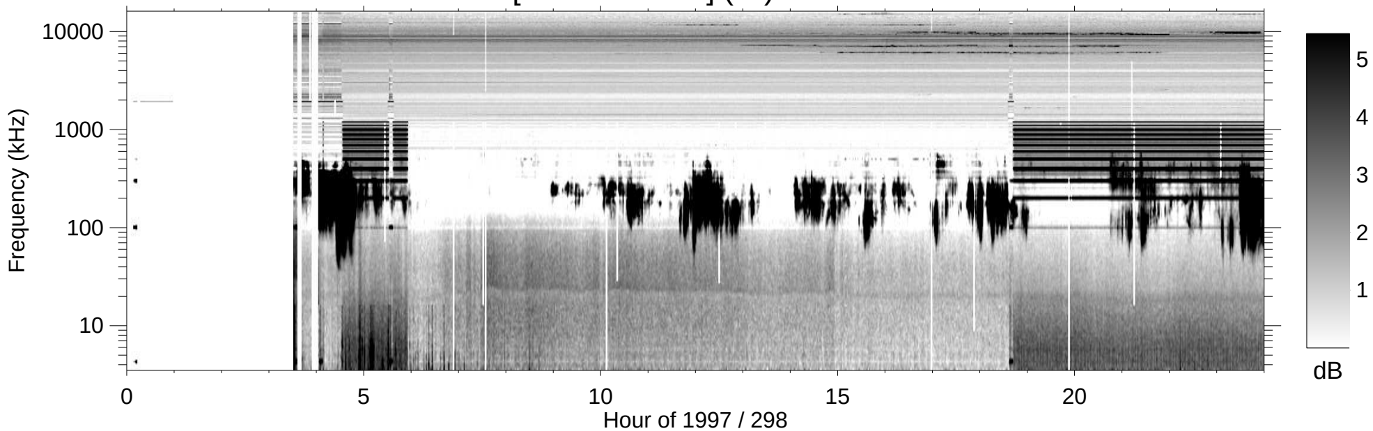
RPWS [ABCH1H2/Ex] (-B) 1997/10/25
