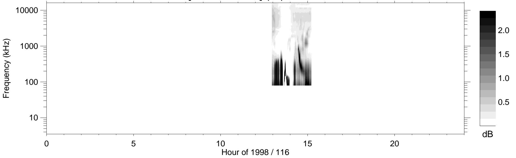
RPWS [ABCH1H2/Ex] (-B) 1998/04/26
