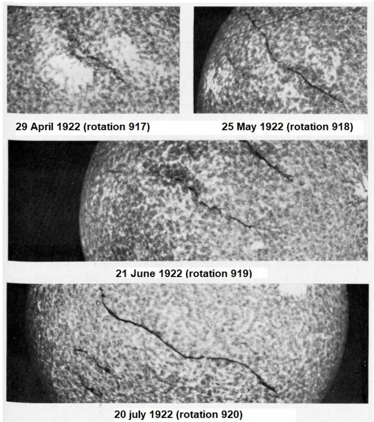
Figure 30. An extremely long filament observed during several rotations. It started to form during rotation 915 (not shown). The length at rotation 920 exceeds one million kilometres. After d’Azambuja & d’Azambuja (1948).
