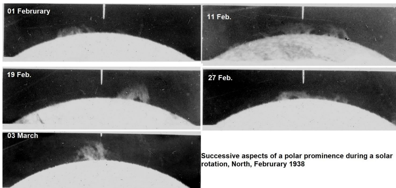
Figure 15. Evolution during the solar rotation of a polar prominence (February 1938). Father Angelo Secchi (1818-1878) wrote in his book “Le Soleil” : “Prominences exhibit so various shapes that it is impossible to describe them with any exactitude”... Courtesy Paris Observatory.
