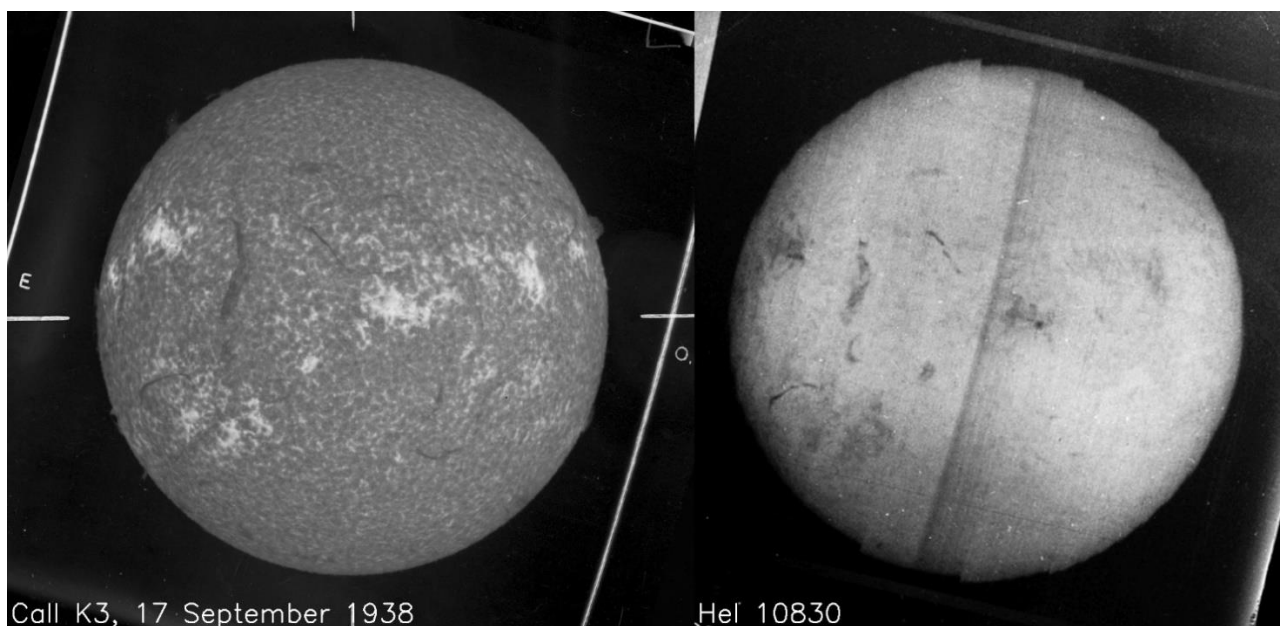
Figure 23. The first observation of the infrared Hel 10830 Å line (right), where both filaments and plages appear darker than the quiet Sun. Call K3 (left) is given for comparison. 17 September 1938. Courtesy Paris observatory.
