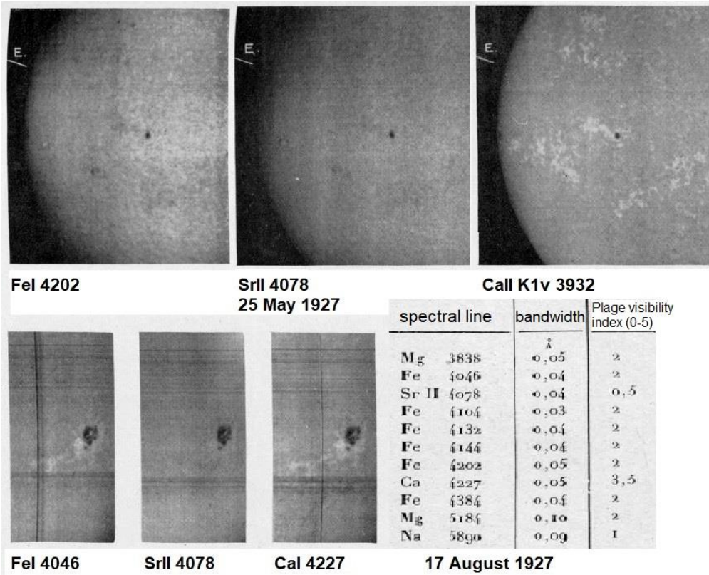
Figure 27. Spectroheliograms in various photospheric lines, compared to Call K1v. After d’Azambuja (1930).
