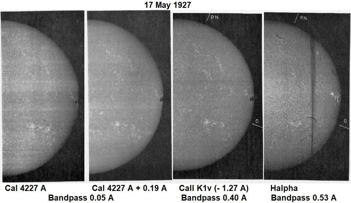
Figure 26. Spectroheliograms of the Cal 4227 Å line, compared to Call K1v for the photosphere (at right, for reference, the chromospheric Hα line). After d’Azambuja (1930).
