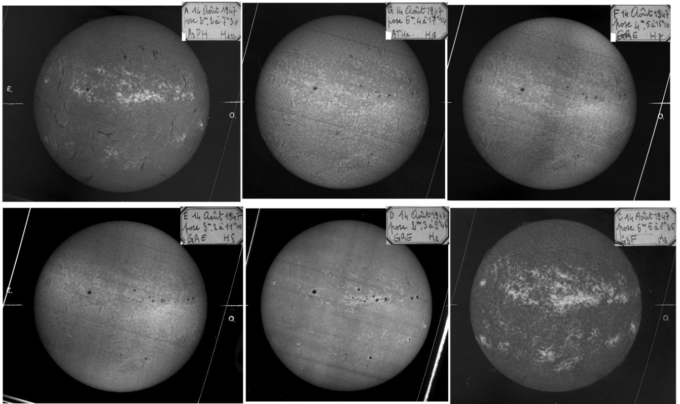
Figure 20. The Balmer series H\alpha , H\beta , H\gamma , H\delta and H\epsilon of Hydrogen, 14 August 1947, and the Call K3 spectroheliogram for comparison. H\alpha is chromospheric, but H\delta and H\epsilon are rather photospheric. Courtesy Paris Observatory.
