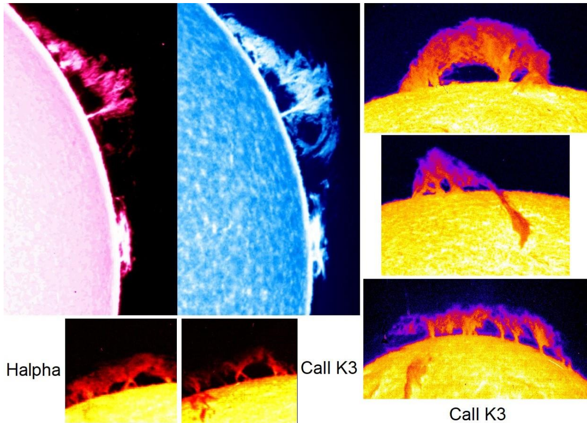
Figure 11. Various aspects of solar prominences in H\alpha and Call K, observed with Meudon spectroheliographs during the first half of the twentieth century (false colours, rainbow coding). Courtesy Paris observatory.
