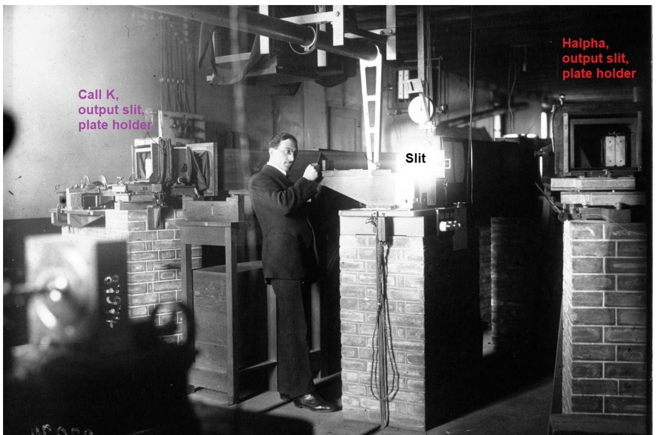
Figure 3. The spectroheliographs with Lucien d'Azambuja in 1921 (Courtesy Gallica/BNF, Meurisse agency).
