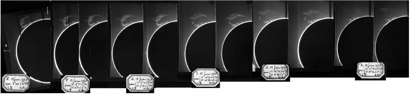
Figure 31. Instability of a solar prominence at the limb observed in Call K3 on 18 June 1925 (08:46 to 11:23 UT) with Meudon spectroheliograph; an artificial moon was masking the solar disk. Courtesy Paris observatory.
