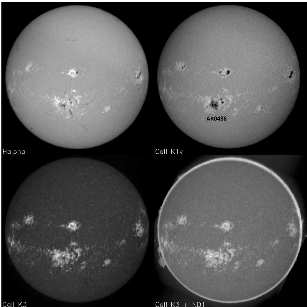
Figure 10. Typical spectroheliograms after WW2 (example of 28 October 2003, the day of a massive X-class flare). H \alpha for the chromosphere (filaments, plages); CaII K1v for the photosphere (sunspots, faculae); CaII K3 for the chromosphere (filaments, bright plages); CaII K3 long exposure time for prominences and limb with a neutral density attenuator ND1 (10% transmission) superimposed on the solar disk. Courtesy Paris observatory.
