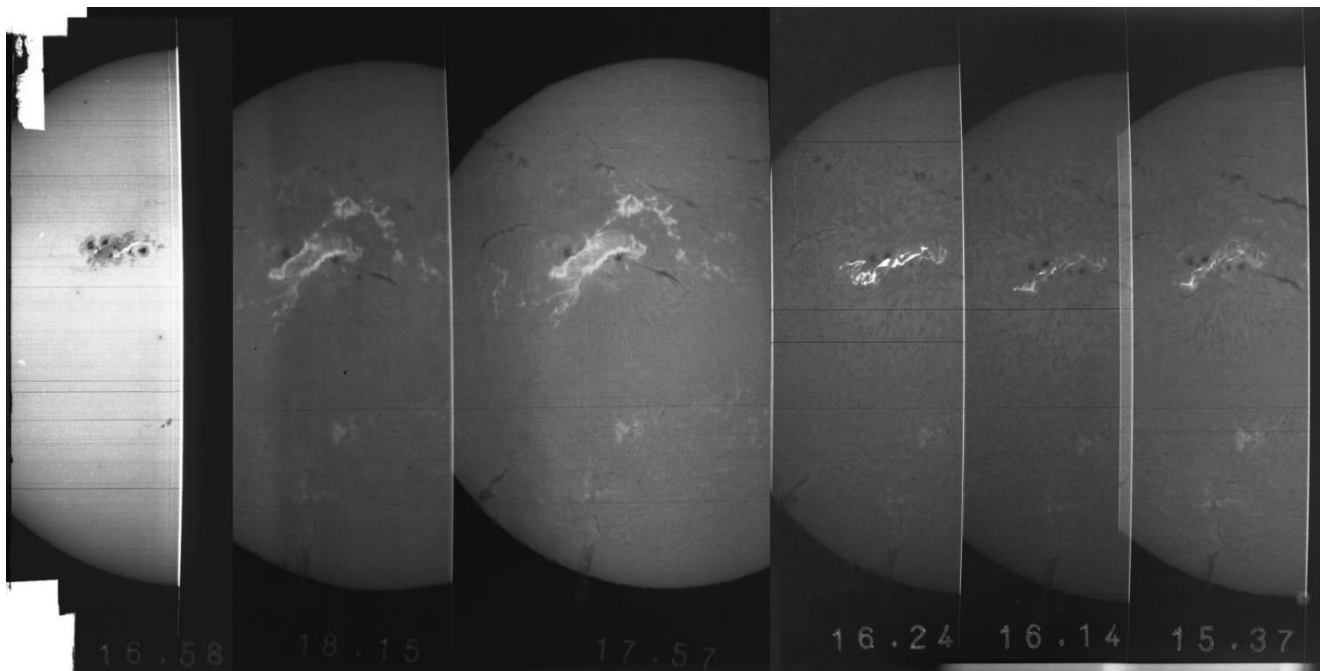
Figure 34. The major two-ribbon solar flare of 25 July 1946 observed in H \alpha with Meudon spectroheliograph (the times are, from the right to the left, 15:37, 16:14, 16:24, 17:57, 18:15 UT). The leftmost image at 16:58 UT was got in the HeI D3 5876 Å line. The short-duration flash phase (lasting minutes) occurred at 16:14 UT. Two bright ribbons (17:57, 18:15 UT) formed during the long-duration gradual phase (lasting hours) and corresponded to the impact of energetic particles on the chromosphere. Courtesy Paris observatory.
