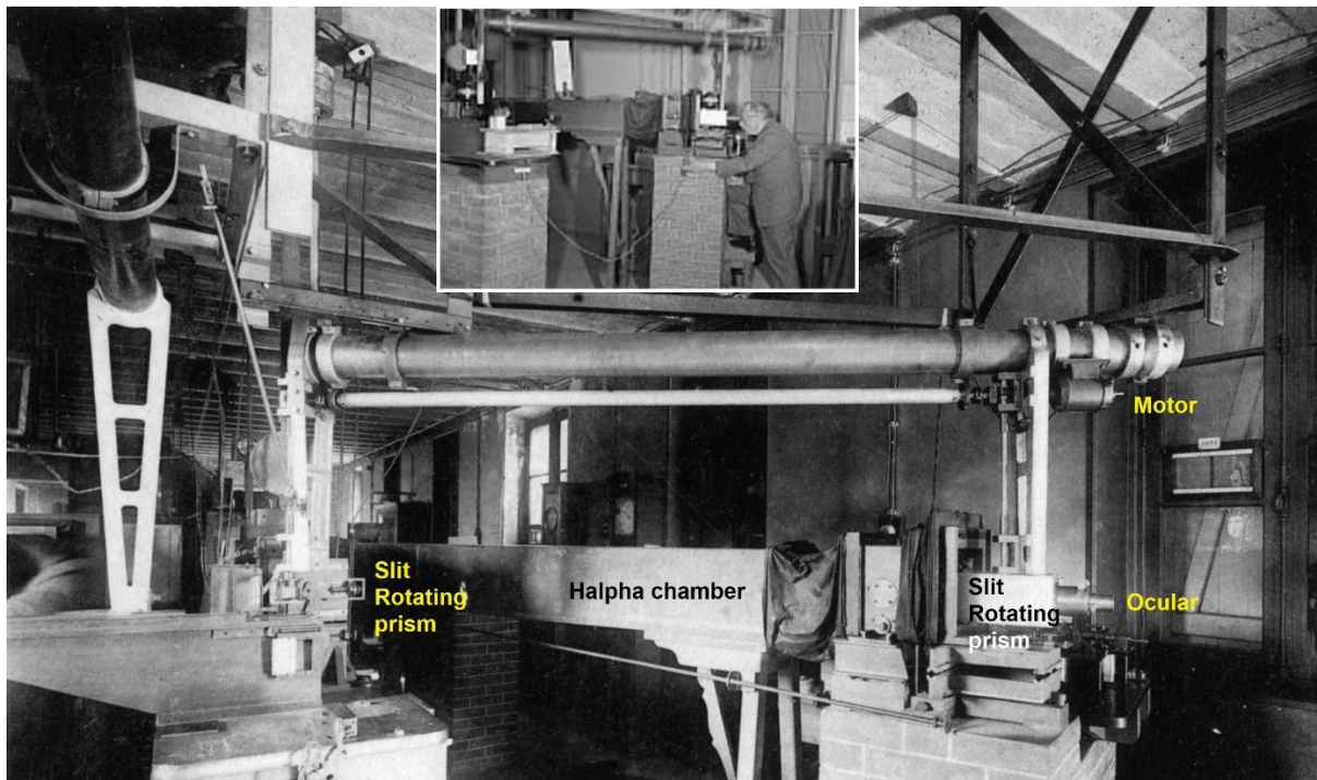
Figure 5. The visual spectrohelioscope in the fifties with L. d’Azambuja in the stamp (courtesy Paris Observatory).
