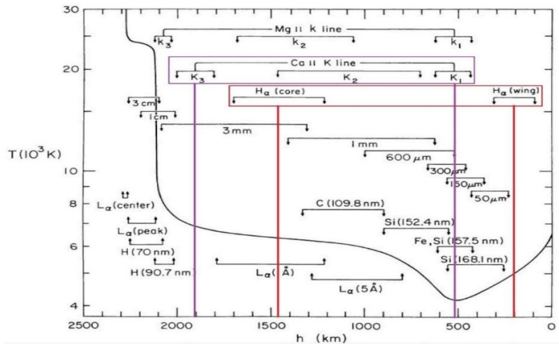
Figure 6. Formation heights (in abscissa) of various solar spectral lines. The cores of H \alpha and Ca II K (named K3) form respectively at about 1500 km and 1900 km in the chromosphere (the layer from 500 km to 2100 km with increasing temperature). The Ca II K2 peaks ( K3 \pm 0.2 \text{ \AA} ) form in the low chromosphere (1000 km), while the wings of H \alpha and Ca II K (named K1, i.e. K3 \pm 1.3 \text{ \AA} ) form respectively at about 200 km and 500 km in the photosphere (the 500 km layer above the surface with decreasing temperature). The Mg II k line in UV (observed by the IRIS/NASA spectrograph in space) looks like Ca II K (after Vernazza et al, 1981).
