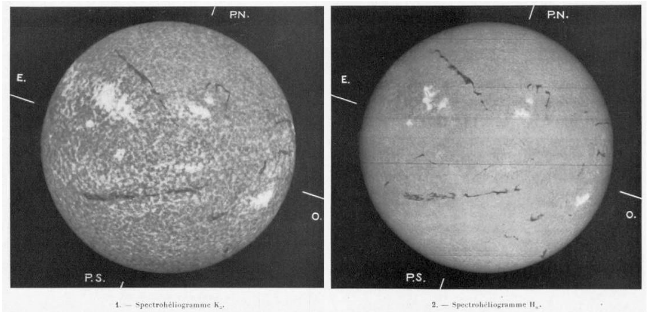
Figure 29. Long filaments of 26 May 1930 in Call K3 (left) and H \alpha (right). After d’Azambuja & d’Azambuja (1948).
