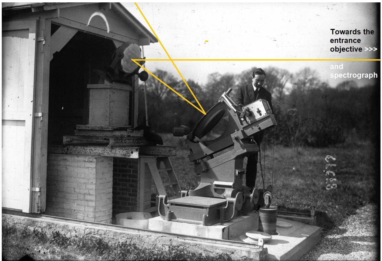
Figure 2. The two-mirror coelostat with Lucien d'Azambuja in 1921 (Courtesy Gallica/BNF, Meurisse agency).
