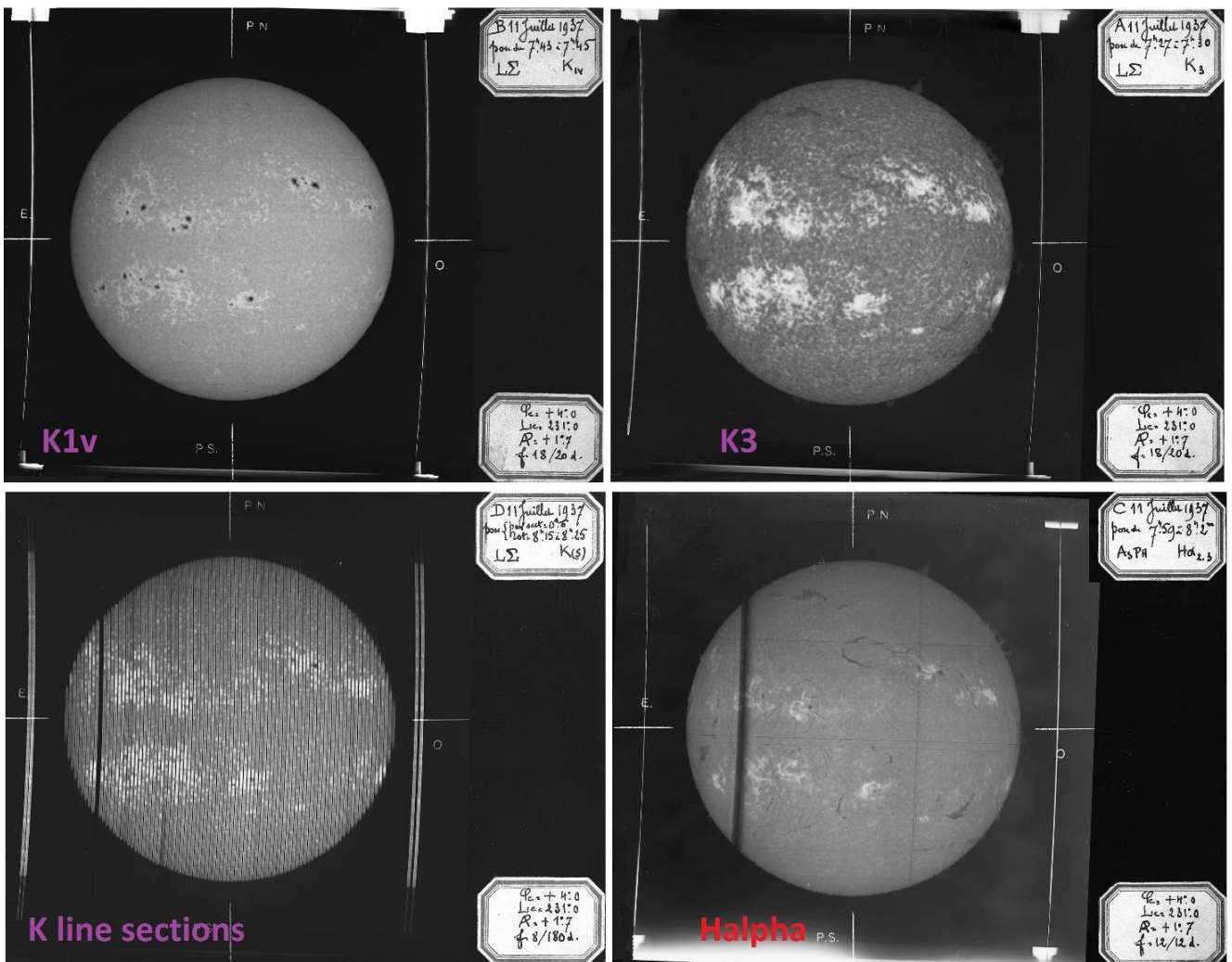
Figure 7. Typical spectroheliograms of the period 1919-1939 (example of 11 July 1937). Call K1v for the photosphere (sunspots, faculae); Call K3 for the chromosphere (filaments, bright plages); Call K line profiles (cross sections of the Sun by 22'' steps for Dopplershift measurements); H \alpha for the chromosphere (filaments, plages). Courtesy Paris observatory.
