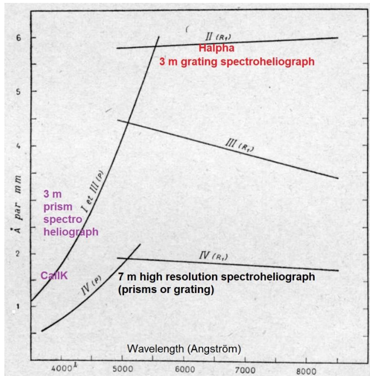
Figure 16. Dispersion of the various spectroheliographs. 3-metre spectrographs n°I (prisms) and n°II (grating) were used only for systematic observations, respectively for CaII K and H \alpha lines. The high dispersion 7-metre spectroheliograph n°IV (3 prisms or plane grating) was used only for research work. After d'Azambuja (1930).
