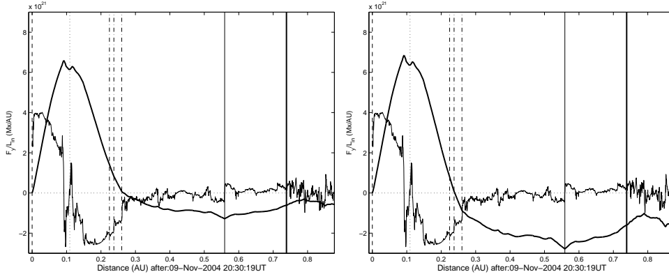
Figure 3. Component of \vec{B} perpendicular to both the trajectory of the spacecraft and to the cloud axis ( B_{y,cloud} , thin line curve) and accumulated magnetic flux of this component per unit length ( F_y/L_{in} , thick line curve). The dotted vertical line marks the cloud center (Nov. 10, 02:02 UT). Left and right panels correspond to computation of F_y/L_{in} without ( L(t) = L_{in} ) and with axial expansion (Equation 4), respectively. In both panels the cloud orientation was taken as \theta = -10^\circ and \varphi = 275^\circ . The vertical lines indicate the same positions as in Figures 1 and 2.
