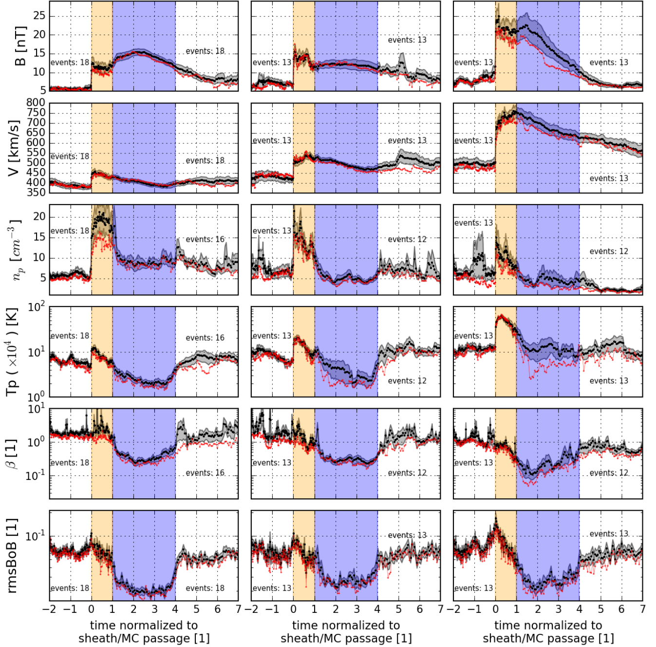
Fig. 4. Average profiles (black lines) distributed in three columns for the three subsets of events. Left: slow ( V < 450 km/s), middle: medium ( 450 km/s < V < 550 km/s), and right: fast MCs ( V > 550 km/s). The black line represents the average value, the grey band represents the error of the mean and the red line represents the median values in each time bin. As in Fig. 2, for t < 1 , time is normalised with the sheath average radial duration and for t > 1 , time is normalised with the average MC radial duration. Orange delimits the sheath region ( 0 < t < 1 ), and blue the MC region ( 1 < t < 4 ). See the caption of Fig. 2 for more information. From top to bottom the parameters are the means of: magnetic field B , bulk velocity V , proton density n_p , proton temperature T_p , plasma beta \beta and normalised magnetic-fluctuation density rmsBoB , Eq. (1).
