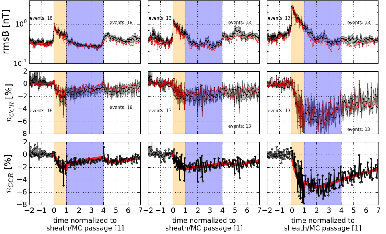
Fig. 6. Superposed epoch for the three subsets of events. Left: slow ( V < 450 km/s), middle: medium ( 450 \text{ km/s} < V < 550 km/s), and right: fast MCs ( V > 550 km/s). First row: mean profiles of magnetic fluctuations rmsB , Eq. (2). Typically, inside the MCs, the fluctuations are the same as in the ambient solar wind. For slow and mid groups, rmsB has higher values in the rear with respect to the ambient solar wind. Second row: mean profiles of GCR intensity n_{GCR} . Before averaging events, the intensity was normalised by the pre-shock level. In the first and second rows the black line represents the average value, the grey band represents the error of the mean and the red line represents the median values in each time bin. Third row: Fitted model (red lines) to the observed average profiles (see Sect. 5.2). See the caption of Fig. 2 for more information.
