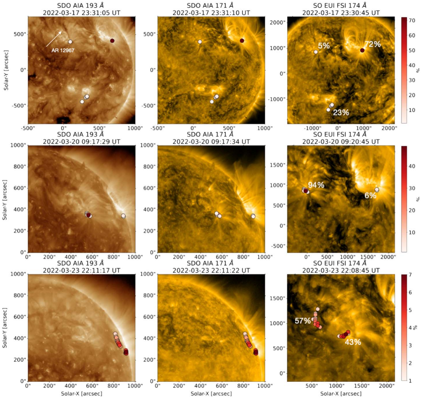
Figure 7. SDO/AIA 193 Å, SDO/AIA 171 Å, and SO/EUV FSI 174 Å images (left to right) on 2022 March 17, 20, and 23 (top to bottom, Sun times) showing connectivities from the MCT at Sun times. This is between 1.5 and 2.25 days earlier than spacecraft times for this data set. Separation angle between SDO and SO is 40^\circ . Colors of circles show the probability of the connectivity (see color-coding on the right side and Section 5). The percentages are the probabilities for each region. The white arrow indicates the open-field corridor of S-web.
